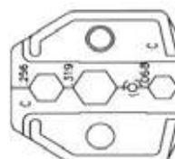
RG58, 59, 62, 6 .256"/.319"/.068"/.213" 6.50/8.10/1.73/5.41mm
