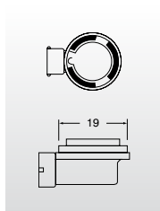
PGJ19-5
