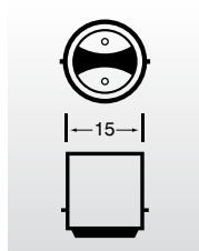
Ba15d
