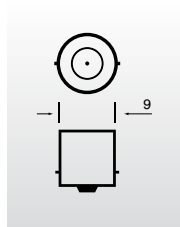
Ba9s
