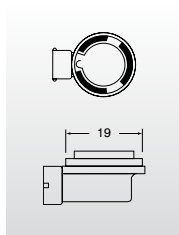
PGJ19-1
