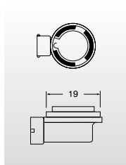
PGJ19-2
