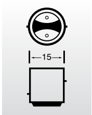
Bay15d
