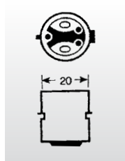
Ba20d
